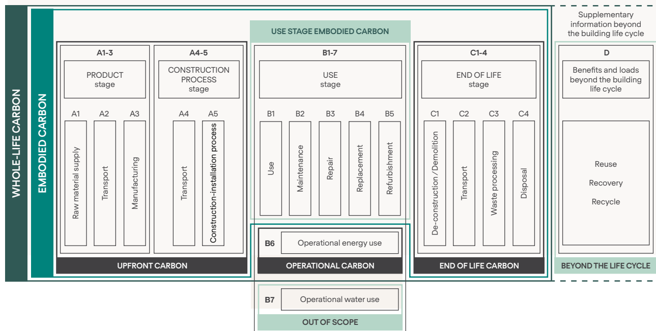
Figure 6 – Embodied carbon life cycle stages.
